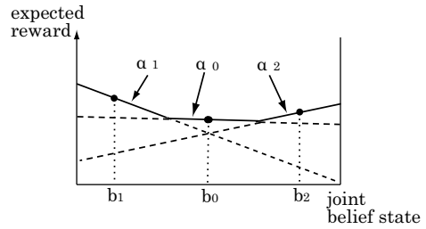
Fig. 3. Value function and \alpha vectors
