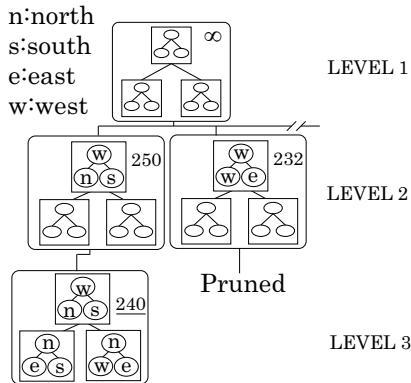
Fig. 2. Execution of SPIDER
