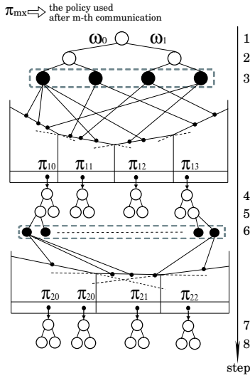
Fig. 4. Policy obtained by LID-JESP-Comm or SPIDER-Comm
